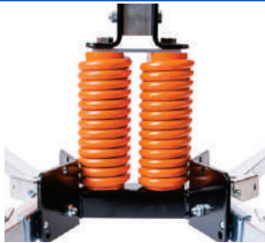
Coil-Spring
